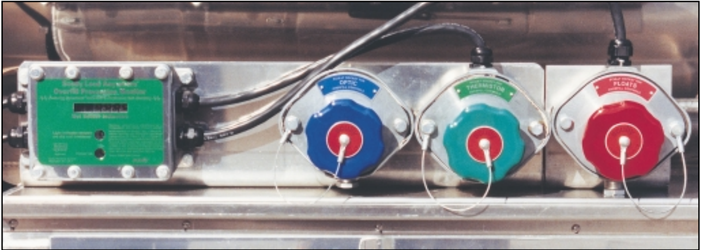
Scully truck mounted control monitor and sockets
